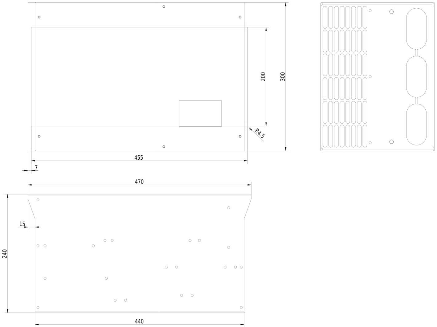
Dimensional drawing V900 - 55kW 4T0550
